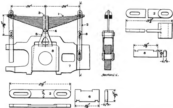
Figs. 1605-1614. Spring Rigging with Slab Front Frame. Atlantic (1-4-2) Locomotive. Pennsylvania Railroad.
